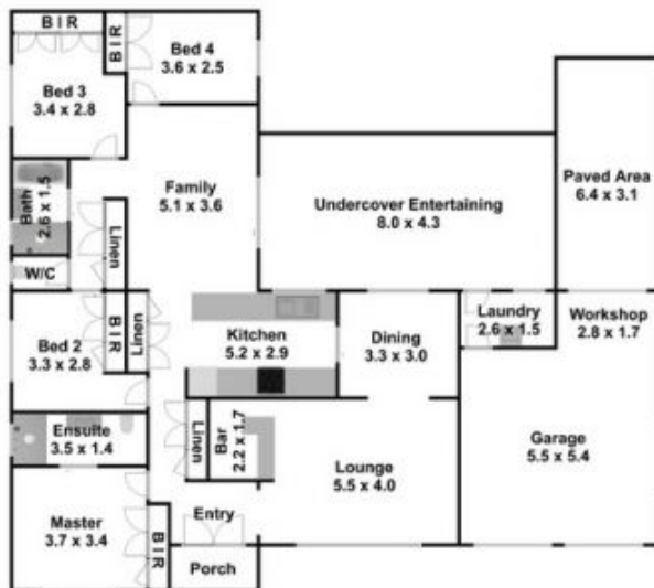
FLOORPLAN
