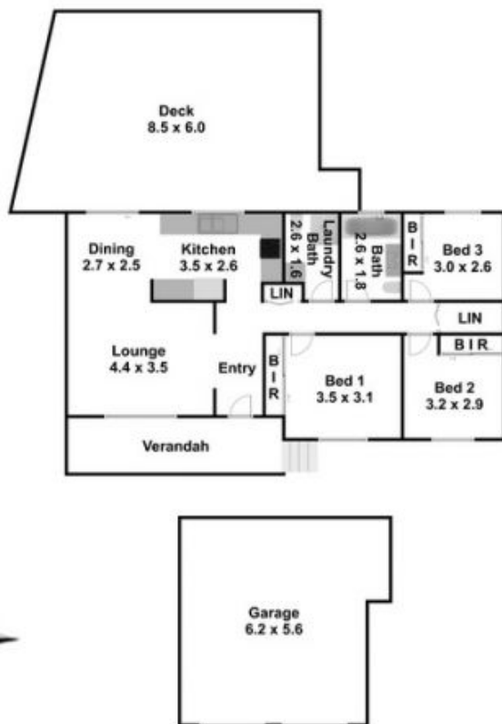
FLOORPLAN
