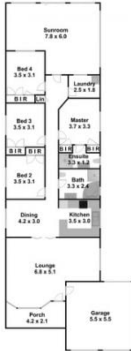
FLOORPLAN
