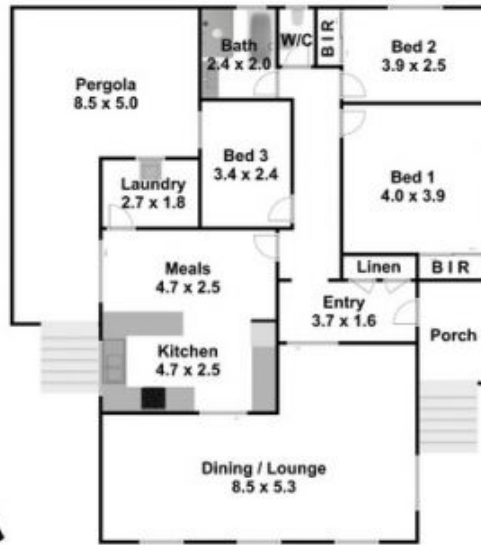
FLOORPLAN
